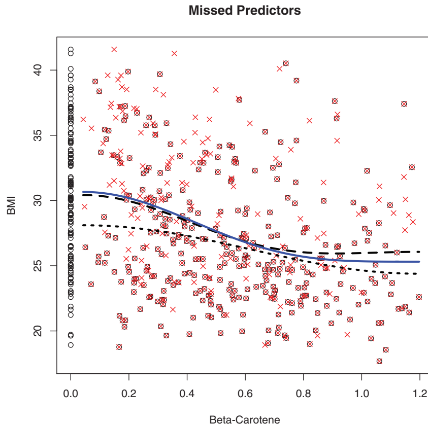
Figure 6. Nonparametric regression for the case of missed predictors. Observations, shown by circles and crosses, are the same as in Figure 3. The solid, long-dashed and short-dashed lines are: the estimate shown in Figure 3b which is based on all underlying observations shown by crosses; the recommended estimate based on data with missed predictors shown by circles; the estimate based on complete cases shown by crossed circles.
