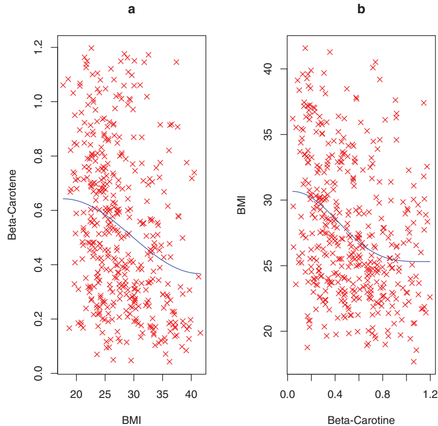
Figure 3. Nonparametric regression estimates for complete data. The same dataset of size n = 441 is shown in both diagrams by crosses, the solid lines show nonparametric regression estimates.
