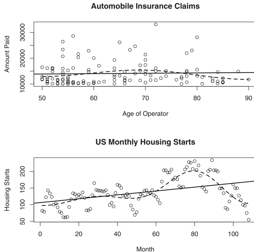
Figure 1. Linear and nonparametric regressions for two classical datasets. Observations are shown by circles, linear and nonparametric regressions by solid and dashed lines, respectively. Sample sizes in the top and bottom diagrams are 124 and 108, respectively.
