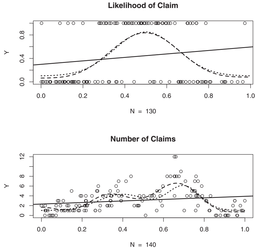
Figure 5. Nonparametric regression, based on complete pairs, for the case of missed responses. Original data is shown in Figure 2. Number N of complete pairs is shown in the diagrams. The short-dashed, solid and long-dashed lines show underlying regression functions, linear and nonparametric regressions, respectively.
