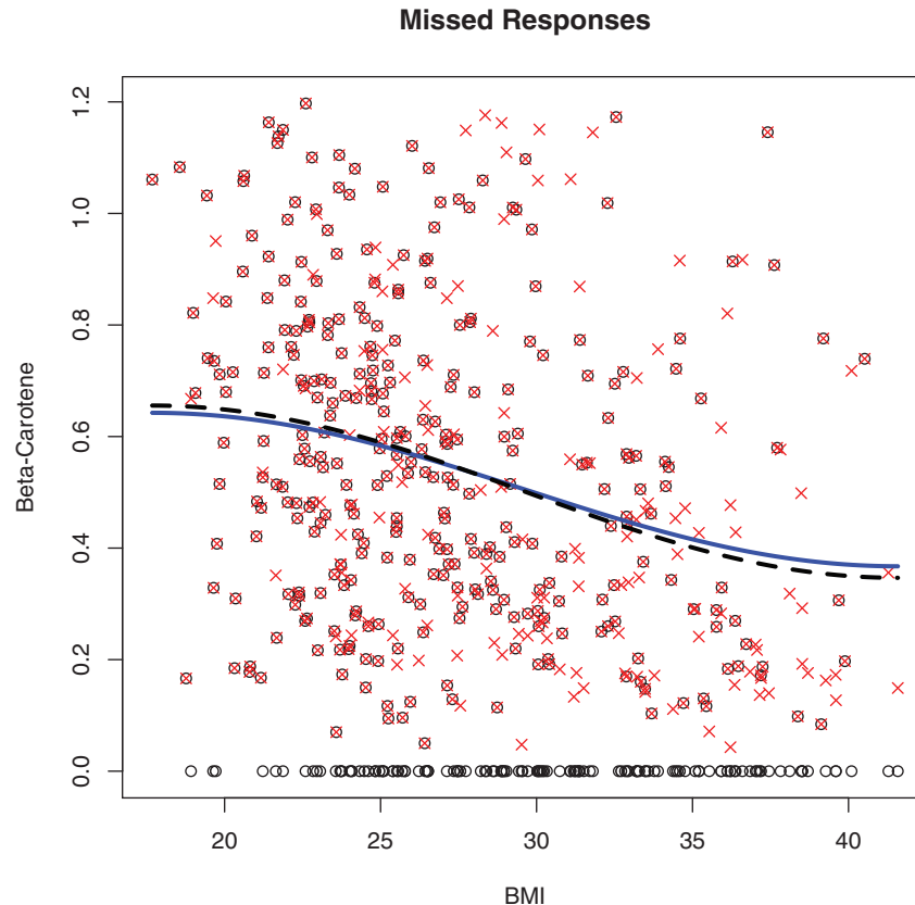
Figure 4. Nonparametric regression for the case of missed responses. Crosses and the solid line are identical to ones in Figure 3a, that is, crosses are n = 441 realizations of (X, Y) for the WHEL breast-cancer data. Then a sample of size n = 441 from Bernoulli A is generated, and circles show realizations of (X, AY) with the number of complete pairs N = 312 . As a result, for the case of missed responses, available complete pairs are shown by crossed circles, incomplete observations are shown by circles with the corresponding (unavailable for statistical analysis) complete pairs shown by crosses. The long-dashed line shows the nonparametric estimate based on complete pairs.
