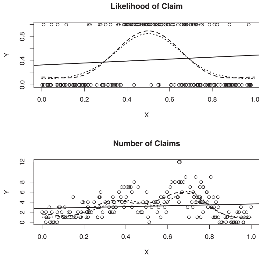
Figure 2. Linear and nonparametric regressions for simulated data, n = 200 . Observations are shown by circles, underlying regression functions, linear and nonparametric regressions by short-dashed, solid and long-dashed lines, respectively.
