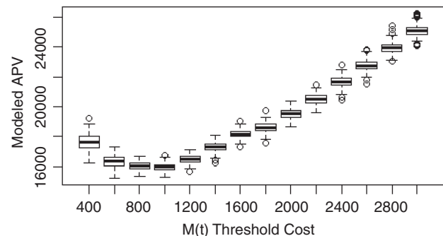
Figure 2.5. Modeled APV: Real discount rate = 3.01%, N_{\text{Sim}} = 200
