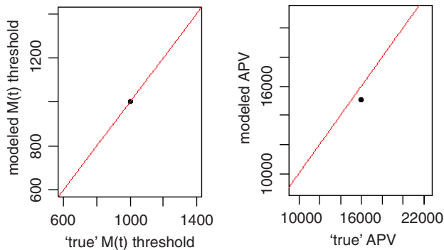
Figure 2.6. True versus modeled M(t) thresholds and minimized APVs for r = 3.01\% , n = 10
