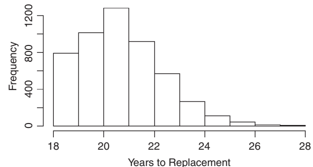
Figure 2.3. Lifespan (time to replacement at threshold of M(t) or time to obsolescence) distribution of asset, generated in module K
