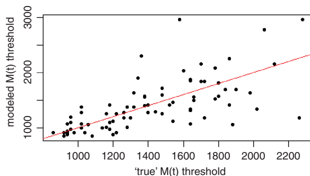
Figure 2.7. True versus modeled M(t) thresholds for r = 3.01\% to 19.01%, n = 10 , generated through 80 iterations of modules A through I
