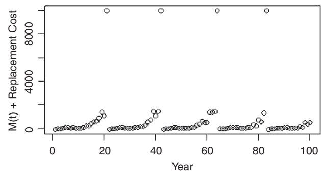
Figure 2.1. Simulated time series of both M(t) and replacement costs for a single asset
