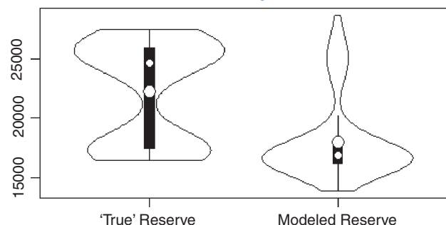
Figure 2.10. Comparison of “true” versus modeled reserves, n = 10 , term = 40 years, r = 0\%
