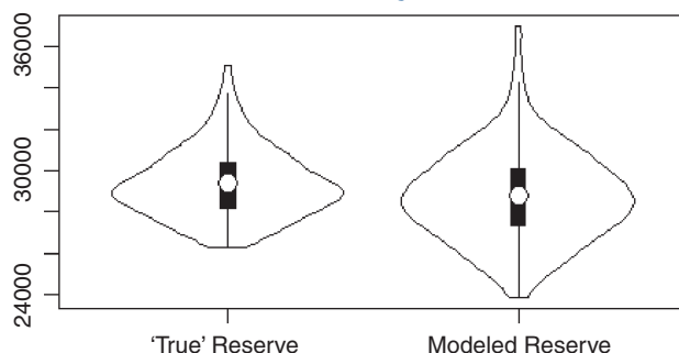
Figure 2.9. Comparison of “true” versus modeled reserves, n = 10 , term = 50 years, r = 0\%
