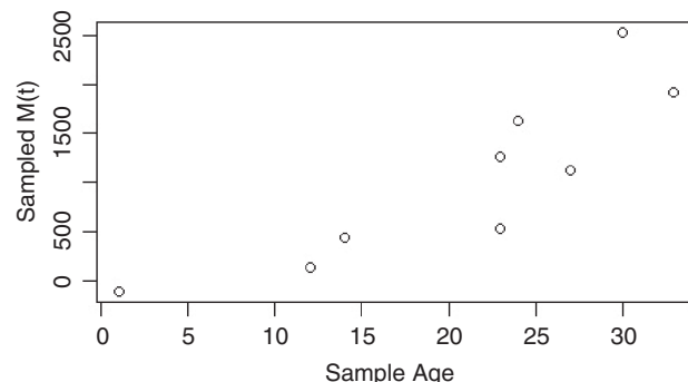
Figure 2.4. A plot of randomly sampled M(t) costs among a set of like assets
