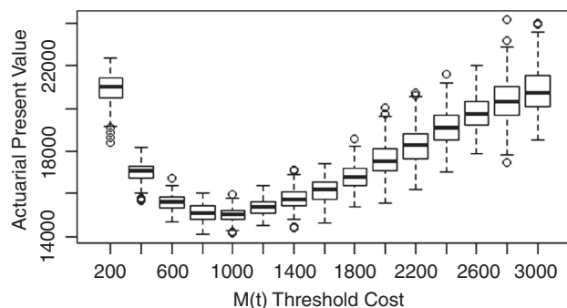
Figure 2.2. “True” APV: Real discount rate = 3.01%, N.Sim = 200
