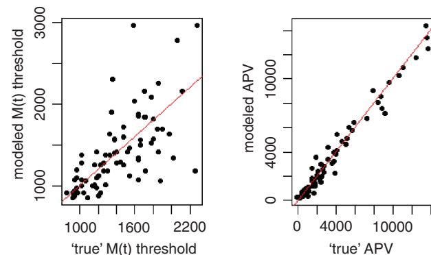
Figure 2.8. True versus modeled M(t) thresholds and minimized APVs for r = 3.01\% to 19.01%, n = 10 , generated through 80 iterations of modules A through I
