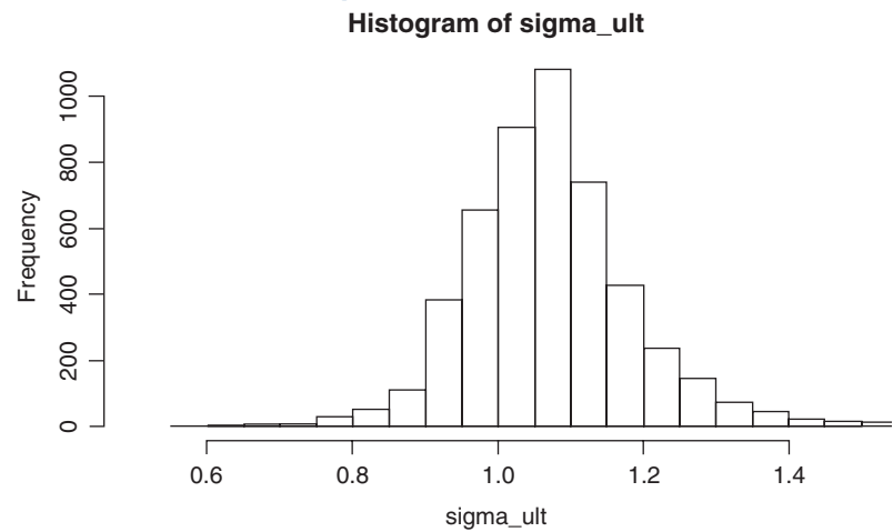
Figure 6. Histogram of posterior \sigma_{ult}
