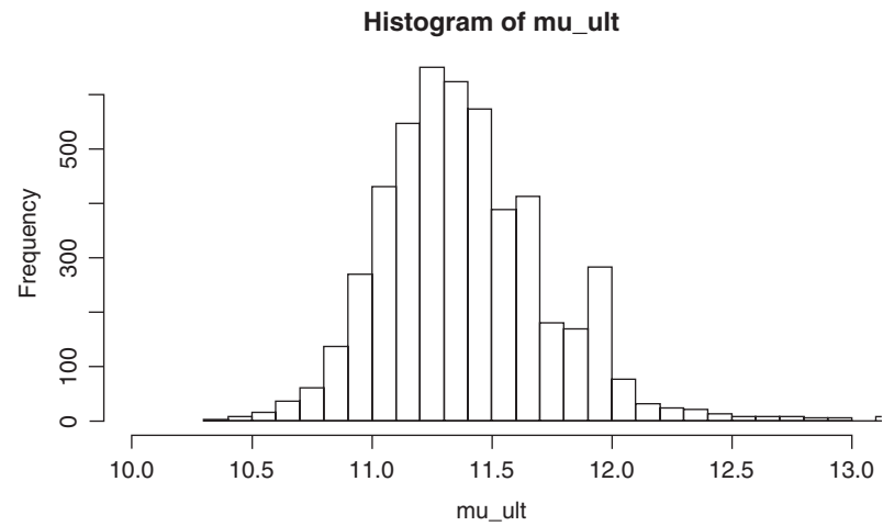
Figure 5. Histogram of posterior \mu_{ult}
