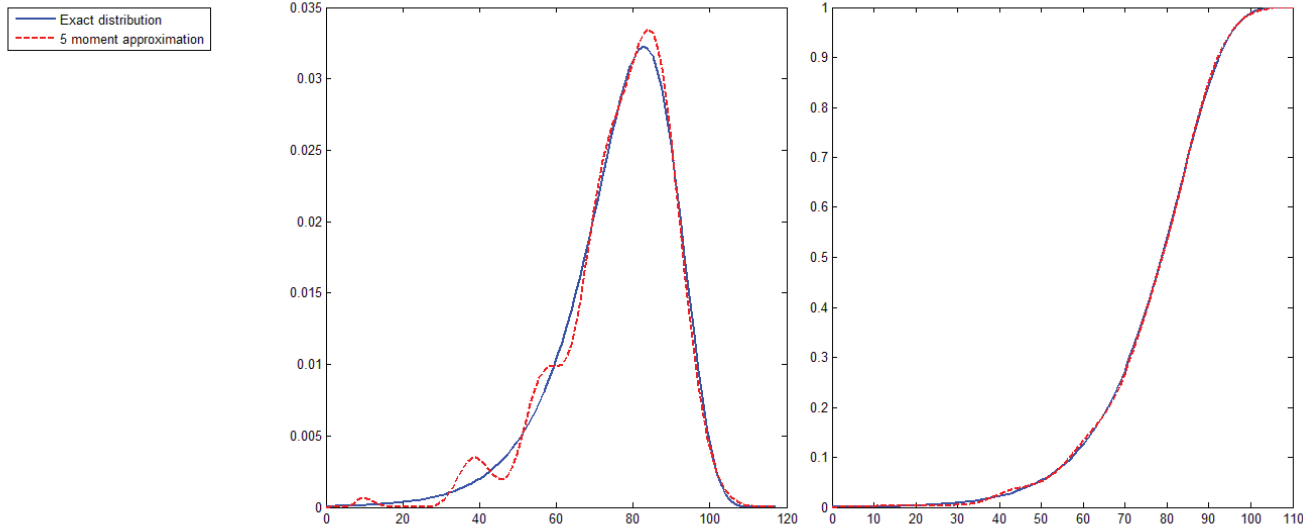
Figure 3. Density (left) and df (right): 5-moment approximation vs Gompertz distribution
