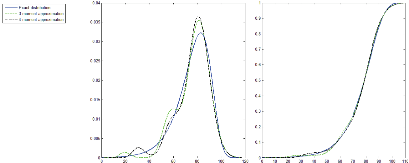
Figure 2. Density (left) and df (right): 3- and 4-moment approximations vs. Gompertz distribution
