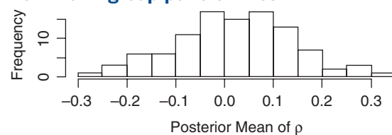
Figure 4.5. Posterior mean \rho s from the 102 within-group pairs of lines
