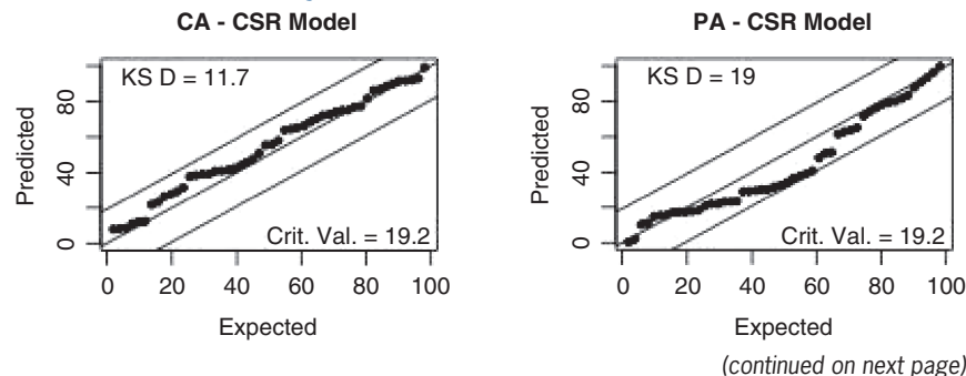
Figure 3.1. Uniformity tests for CSR model
