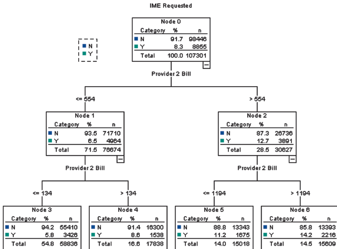
Figure 3A. CART example with seven nodes IME proportion as a function of provider 2 bill
