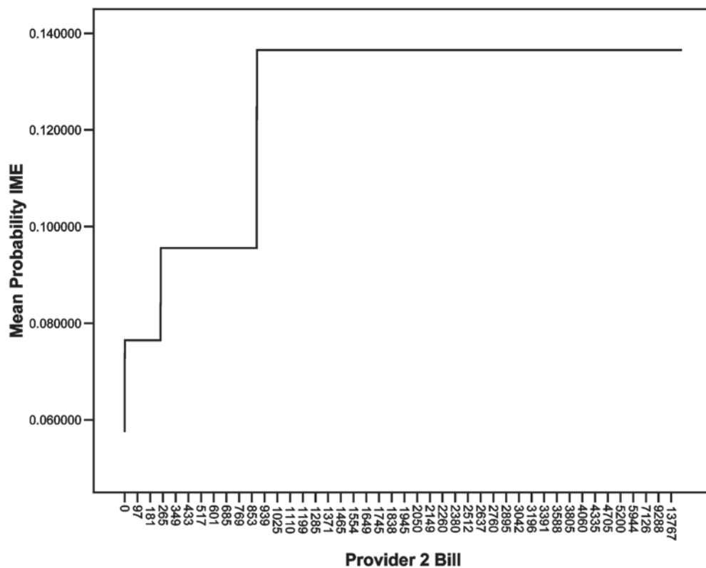
Figure 7. Naïve Bayes predicted IME vs. provider 2 bill
