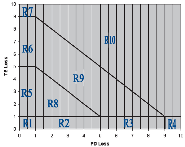
Figure 5. Regions of integration
