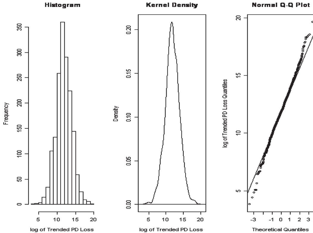
Figure 1. Plots to support the normal assumption for X_1
