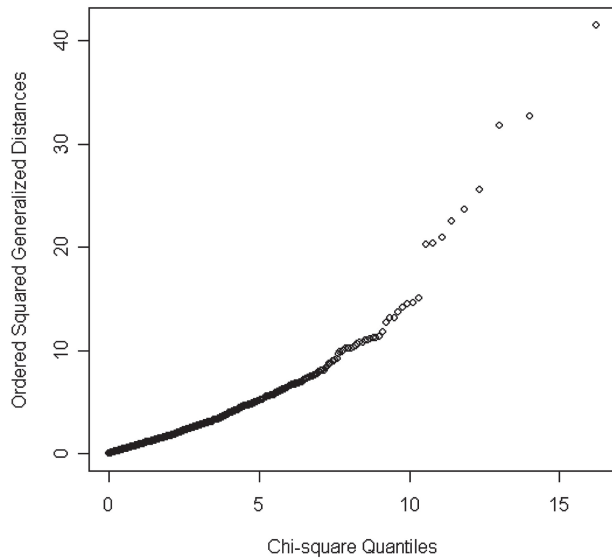
Figure 4. QQ plot for bivariate normality
