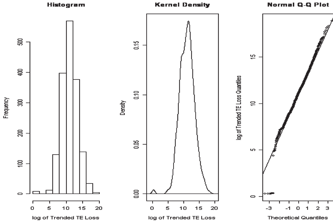
Figure 2. Plots to support the normal assumption for X_2
