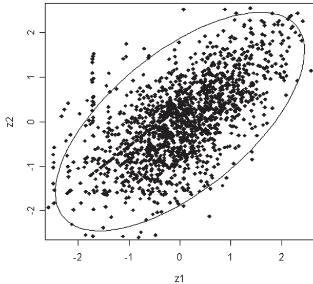
Figure 3. Ellipse with 95% probability coverage
