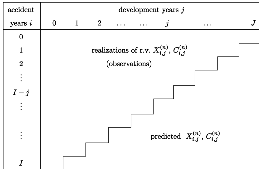
Figure 1. Claims development triangle number n
