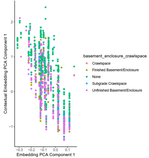
Figure 9. Embedding versus contextual embedding, flood zone, first PCA components, points colored based on crawl space variable.
