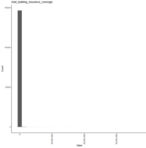
Figure 17. Histogram of the building coverage covariate.
