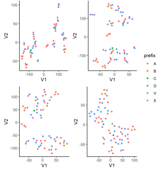
Figure 5. t-SNE plots of learned embeddings of flood_zone in Model 4, with various perplexity values. From left to right, then top to bottom: 2, 3, 5, and 10.
