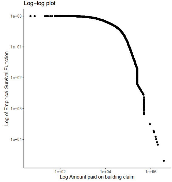
Figure 11. Log-log plot of claim amount.
