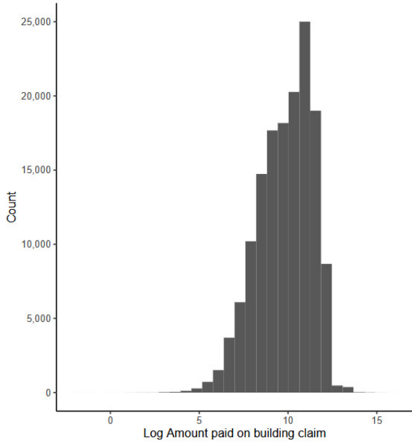
Figure 10. Histogram of the log claim amount.
