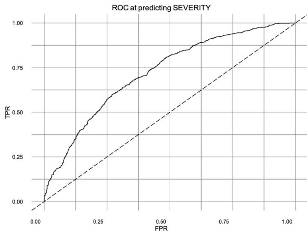
Figure 7. Receiver operating characteristic of the method
