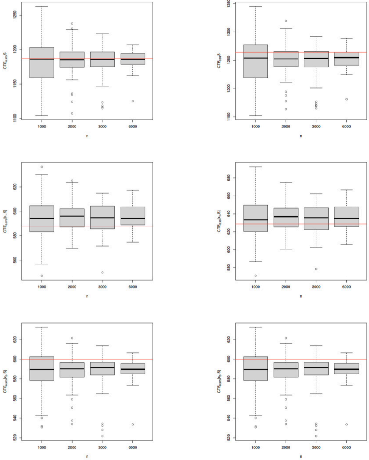
Figure 5. Boxplots for the estimates of CTE_q[S_X] and CTE_q[X_i; S] for i = 1, 2 , and q \in \{0.975, 0.99\} , with the true values are specified by the red reference lines.
