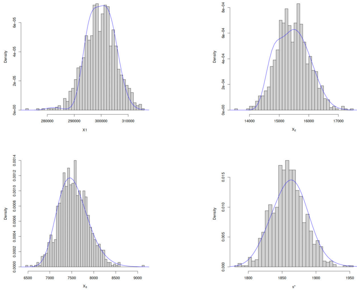
Figure 9. The histograms of liability RV's X_1 , X_2 , X_3 , and the associated standardized sum S^* = X_1/\widehat{\theta}_1 + X_2/\widehat{\theta}_2 + X_3/\widehat{\theta}_3
