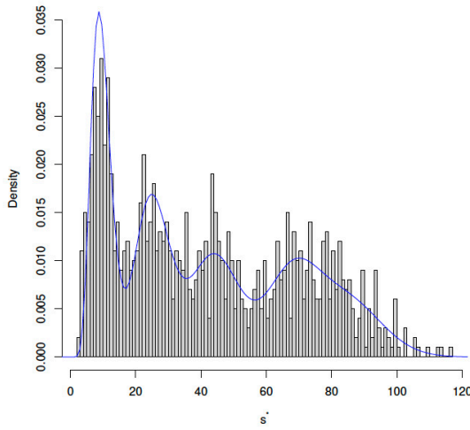
Figure 4. Histogram and QQ plot for the standardized aggregation S^* with the fitted density imposed over the left-hand panel.
