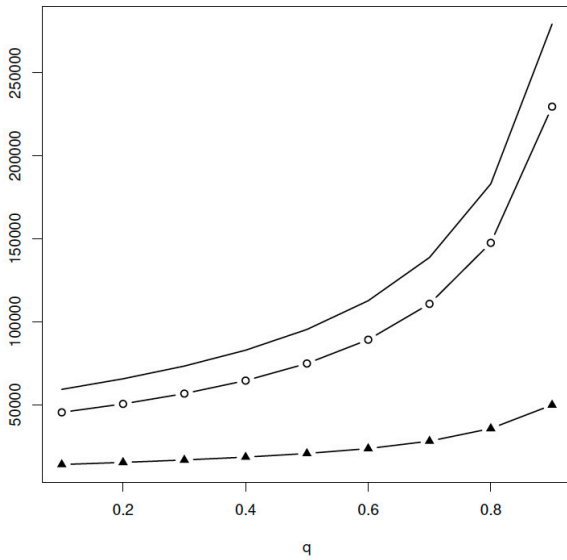
Figure 7. The conditional tail expectations \text{CTE}_q[S_X] , \text{CTE}_q[X_1, S_X] , and \text{CTE}_q[X_2, S_X] , marked by the solid line, dashed line with circles, and dashed line with triangles, respectively.
