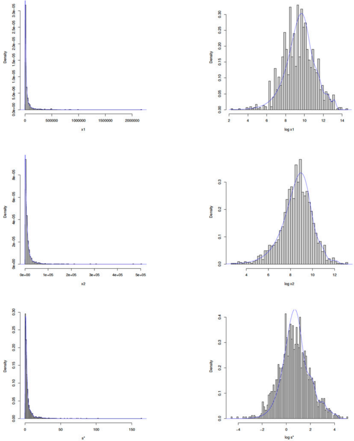
Figure 6. Histograms for X_1 , X_2 , and S^* (left-hand panels) and the corresponding log transforms (right-hand panels) with the fitted MG_2 densities.
