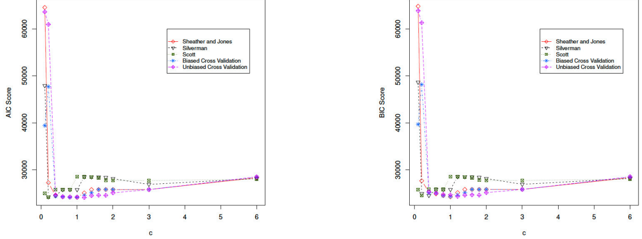
Figure 1. AIC and BIC scores of the MG_2 fitting with varying bandwidth adjuster c \in (0.1, 6)
